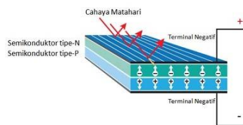
Gambar 2. Sel Surya
