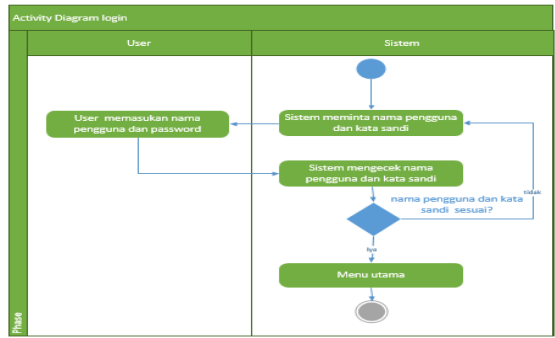
Gambar 4.Activiti Diagram
