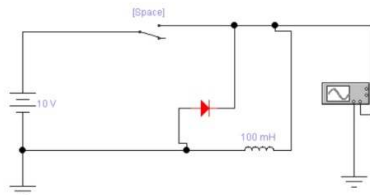
Gambar 3.1 Rangkaian Simulator Uji Dioda Reverse Bias
