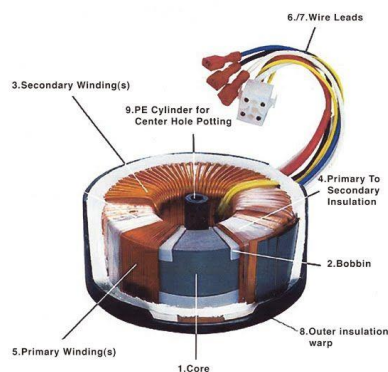
Gambar 5. Bagian-bagian Transformator toroid
