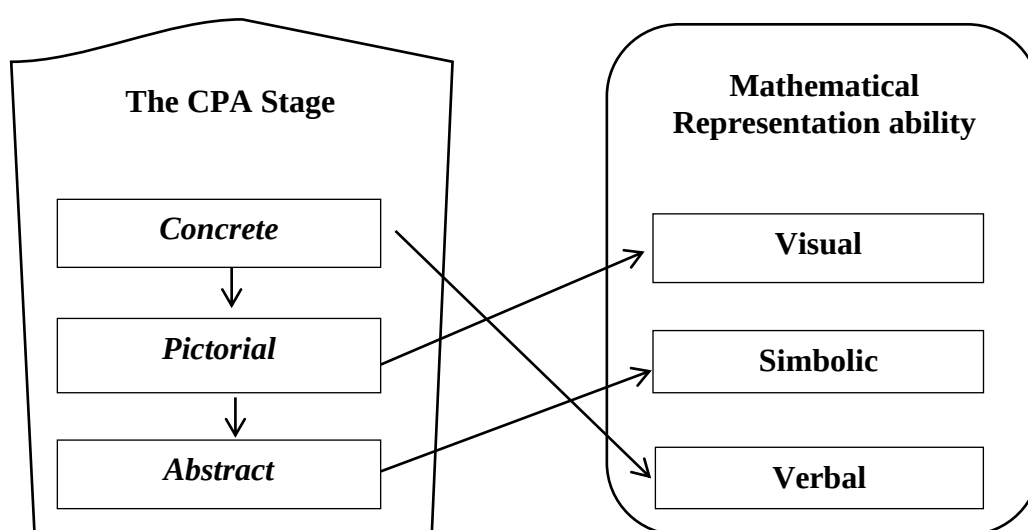
Figure 1 Scheme Framework
